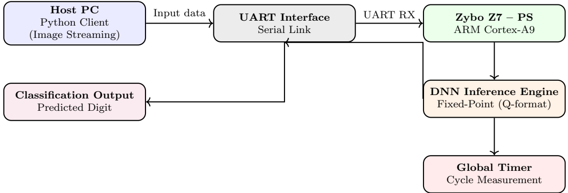
Figure 5.1: UART-based DNN microserver architecture. The host PC streams input data to the embedded platform, which performs fixed-point inference and returns the classification result over the same serial interface.
